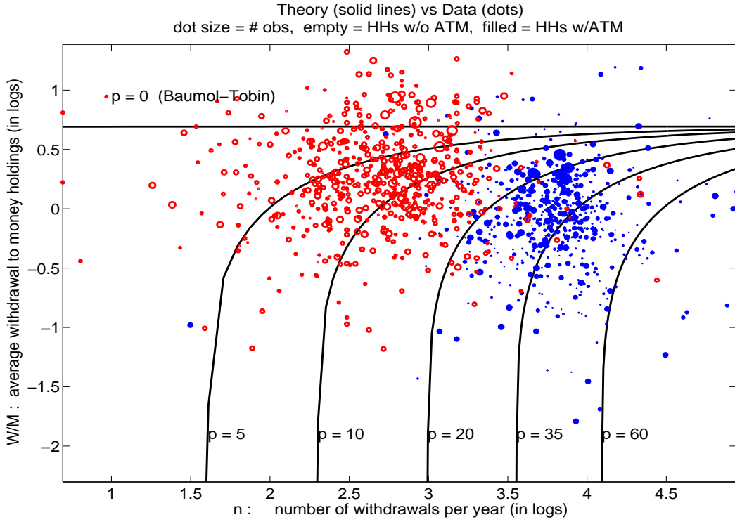
Figure 4: Theory vs. data (province-year mean): W/M, n
