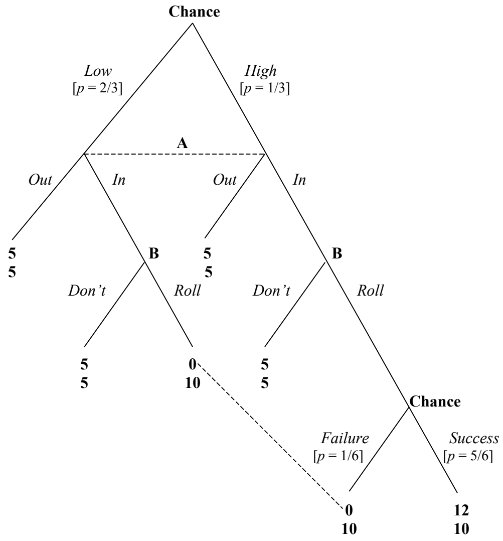
Figure 2: The (5,5)-game
