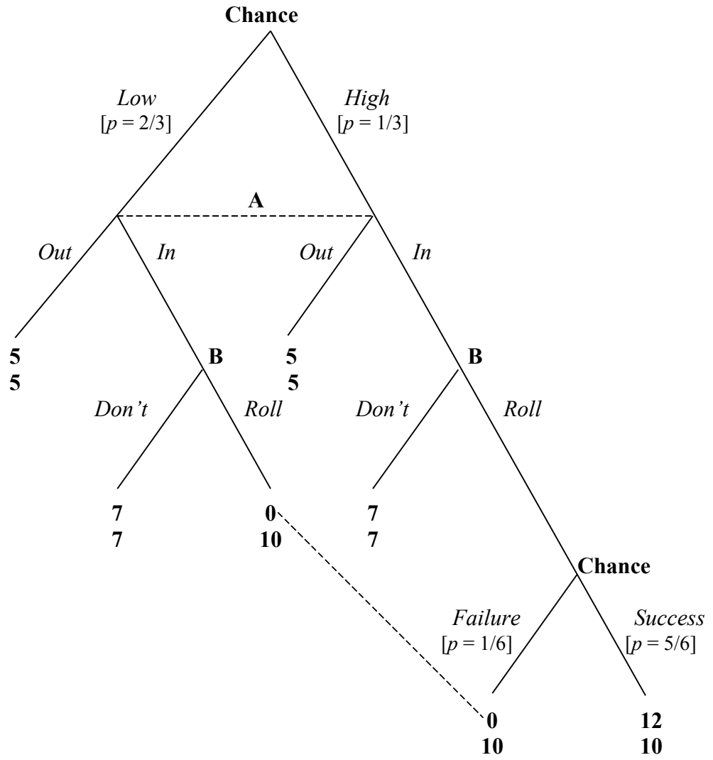
Figure 1: The (5,7)-game
