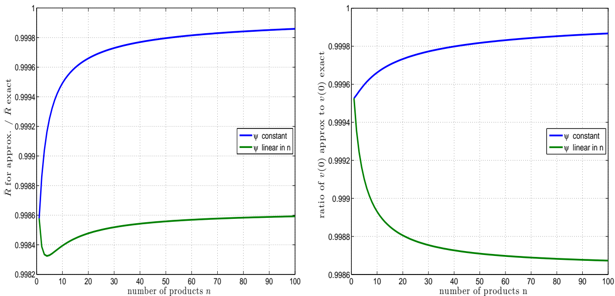
Figure 4: Ratio of \bar{R} 's and of v(0) 's for the approximation relative to the “exact” solution
