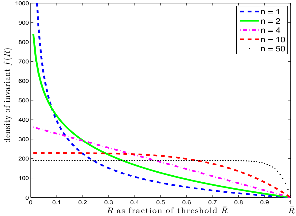
Figure 1: f(\cdot) density of invariant distribution of R , for various choices of n
