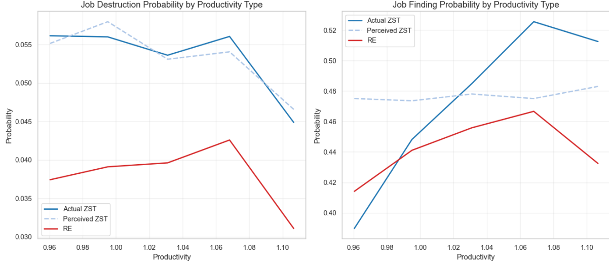
Figure 7: Job Destruction and Job Finding Probability by Productivity Type. The model with ZST workers shows higher job destruction rate than the RE one. Expectations about the job destruction rate are correct for any productivity level, while expectations about the job finding probability result to be stubborn with respect to workers' productivity.
