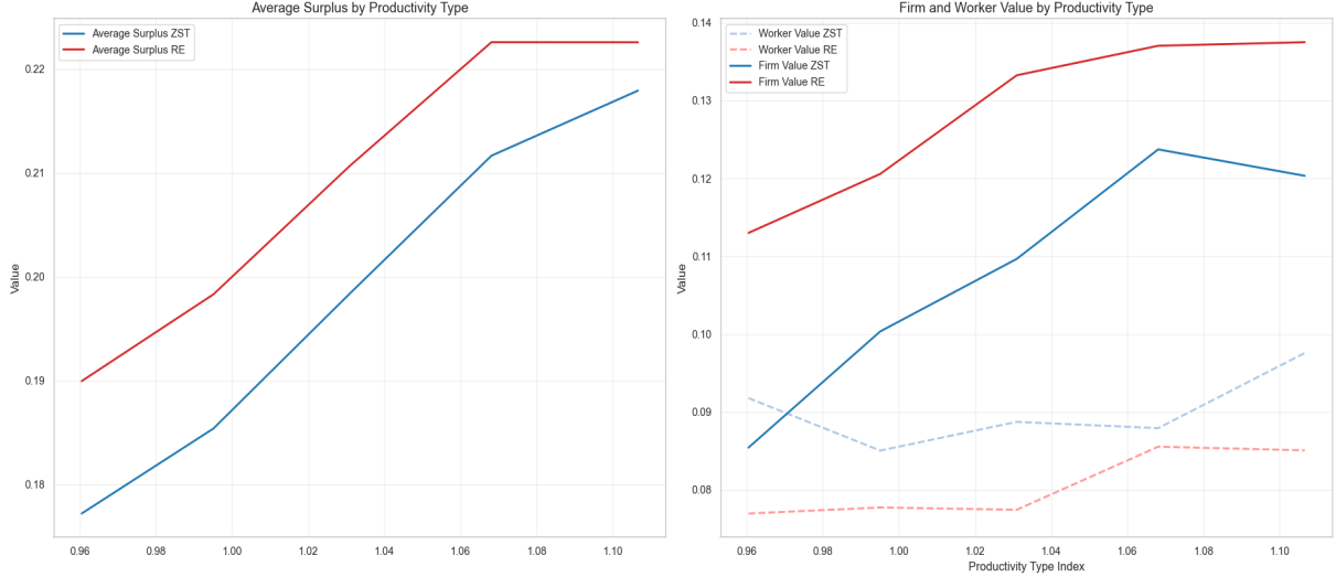
Figure 5: Actual Surplus and Surplus Sharing by Productivity Type. Total surplus is lower in the ZST equilibrium relative to the RE, and this result holds across all the productivity levels (on the left). Moreover, the redistribution effect of ZST varies across productivity levels and it is stronger when productivity is low (on the right).
