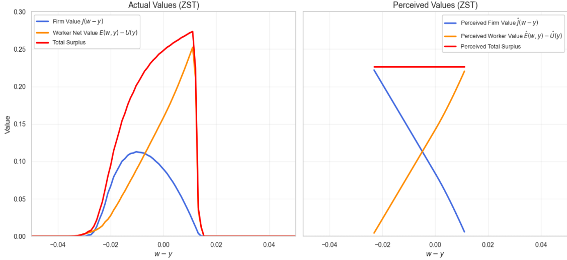
Figure 3: Actual and Perceived Values in the ZST model. The graph on the left shows the actual values of firms and worker, and the resulting actual surplus from matching. The graph on the right shows the values as perceived by the worker, with the resulting perceived surplus that is completely flat.
