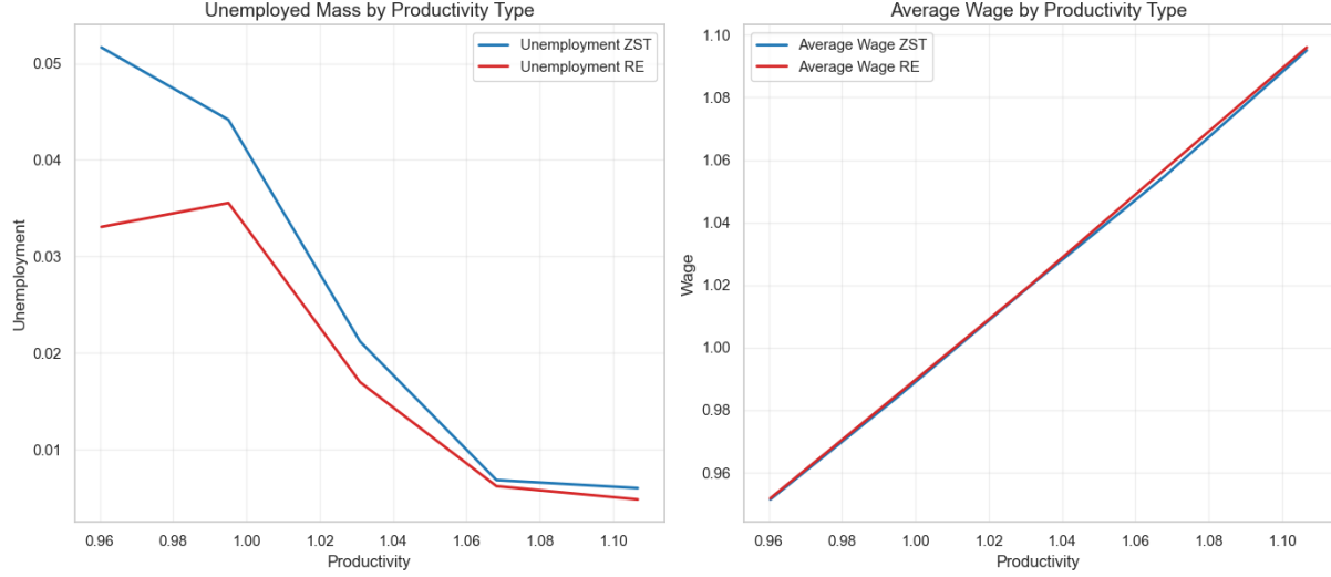
Figure 8: Unemployment Mass and Average Wage by Productivity Type. The ZST economy shows an higher level of unemployment in equilibrium, on the other hand average wages are equal between the two models.
