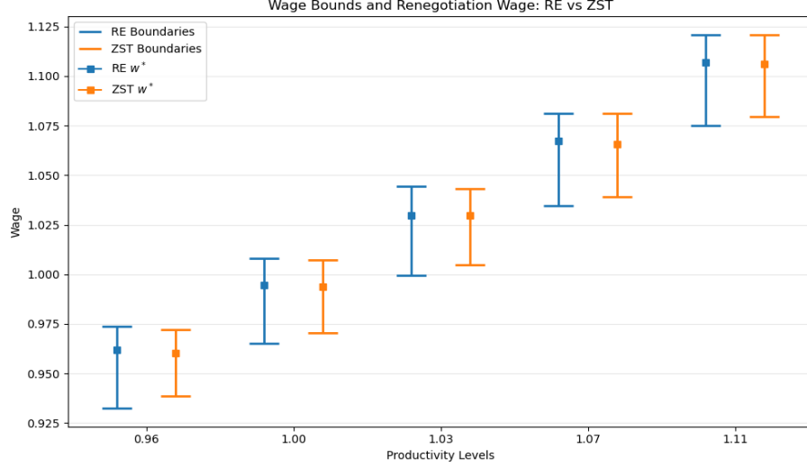
Figure 6: Policy Functions and Renegotiation Wage by Productivity Type. Under ZST the continuation region is shorter, meaning that both workers and firms leave the match earlier than in the RE model. This holds across all productivity levels. Equilibrium wages are similar between the two models.
