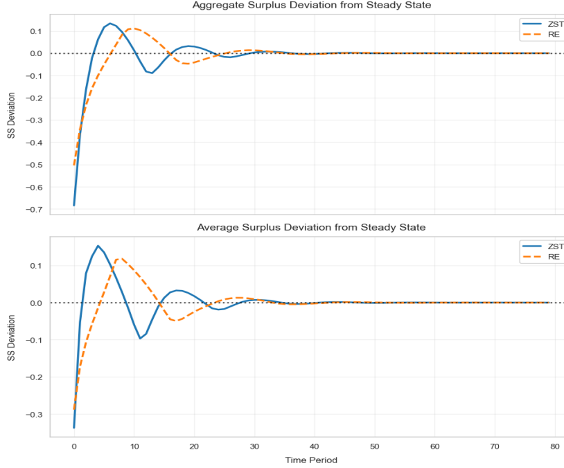
Figure 11: Aggregate and Average Surplus Response to Inflation (deviation from steady state). On impact, both the average and the aggregate surplus decline and respond more in the ZST economy relative to the RE one. While the economies transitions to the steady state after the shock, inflation is temporarily reducing the inefficiencies caused by zero-sum thinking in terms of aggregate surplus.
