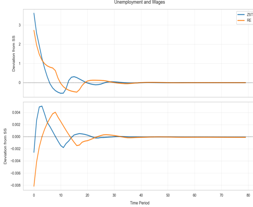
Figure 10: Unemployment Rate and Average Wage Response to Inflation (deviation from steady state). As separations respond more in the ZST model, also unemployment rate increases more on impact relative to the RE economy. Similar response of average wages in both economies.
