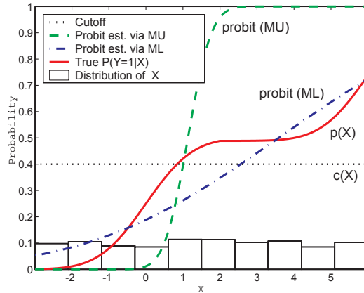
Figure 2: The comparison of utility maximization based estimation and ML
