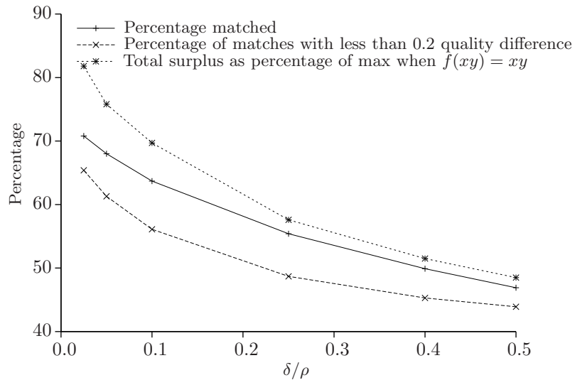
FIGURE 3. Convergence to PAM as \delta/\rho \rightarrow 0
