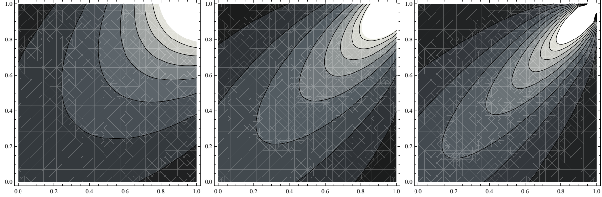
FIGURE 2. Contour maps of steady-state equilibrium matching densities \mu for uniform type densities and three different values of \psi = \delta/\rho : \psi_H = 0.5 (left), \psi_M = 0.1 (middle), and \psi_L = 0.025 (right)
